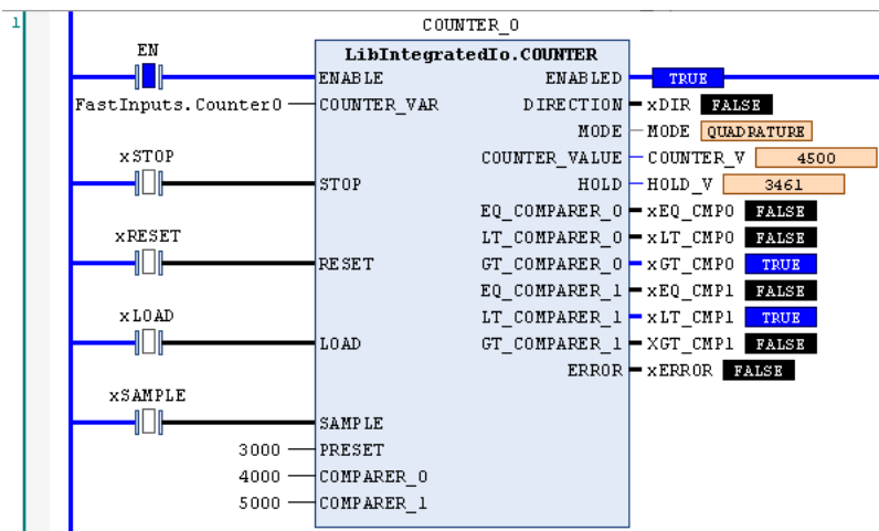
Figura 65: Bloco Funcional LibIntegratedIo.COUNTER
