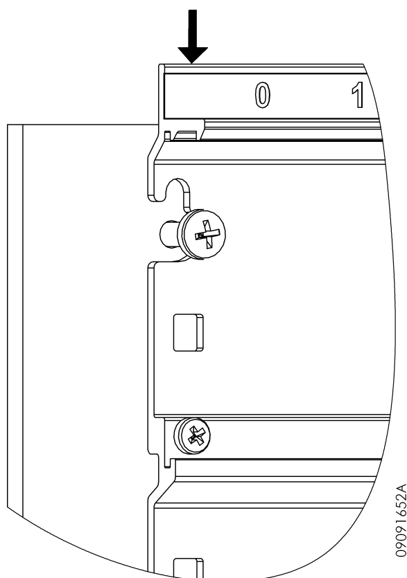
Figure 47: Rack fixation – Keyway fitting
