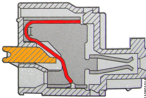
Figure 73: Spring Connection
