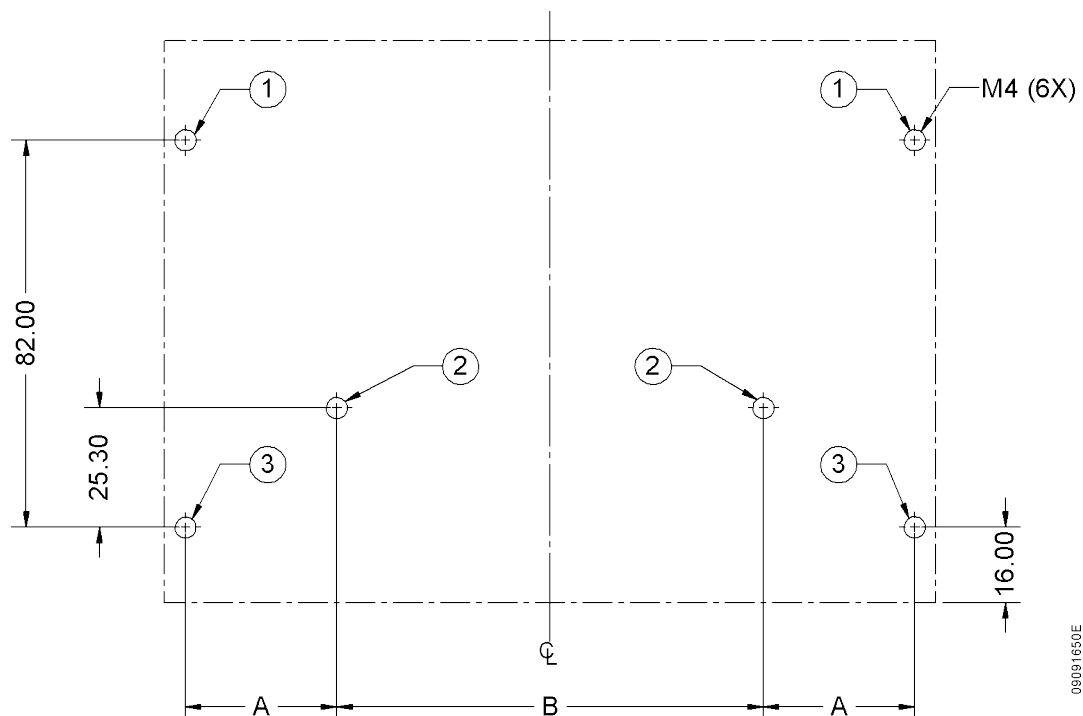
Figure 44: Drilling for Rack Fixation
