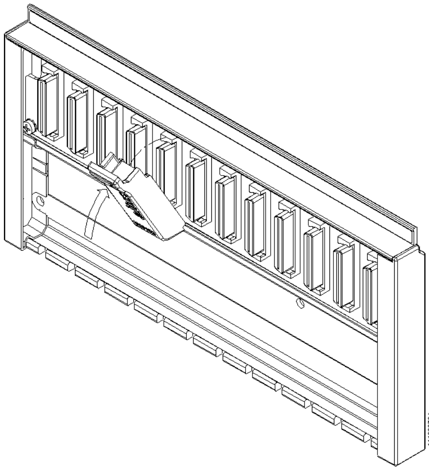
Figure 69: Rack Connector Cover Insertion
