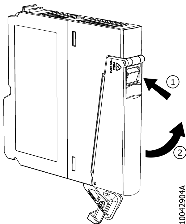
Figure 60: Movement to Remove the I/O Connector Block Nexto Modules
