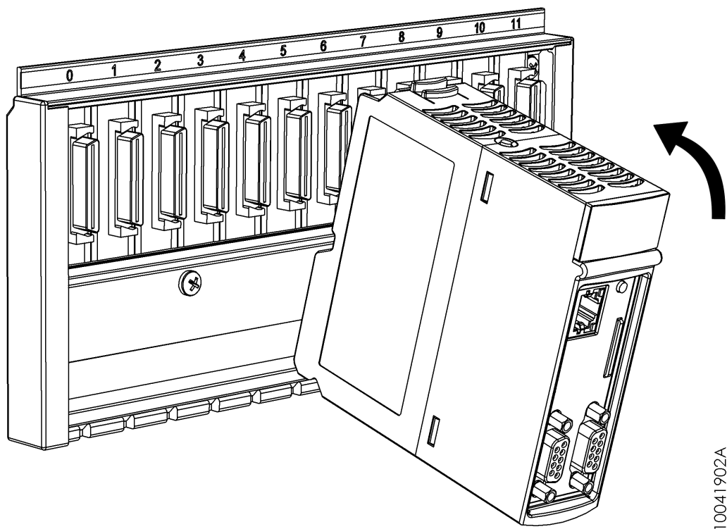
Figure 50: Backplane rack fitting movement
