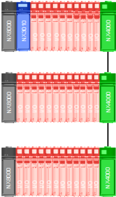
Figure 5: Single CPU with Remote Rack Expansion and Nexto Modules
