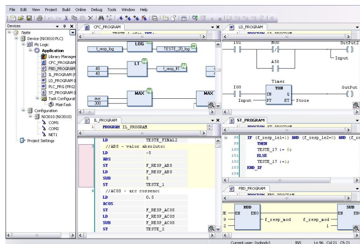
Figure 17: IEC 61131-3 Programming Languages
