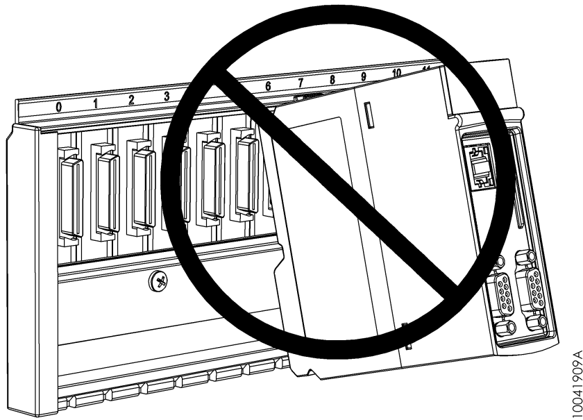
Figure 52: Wrong Insertion Way
