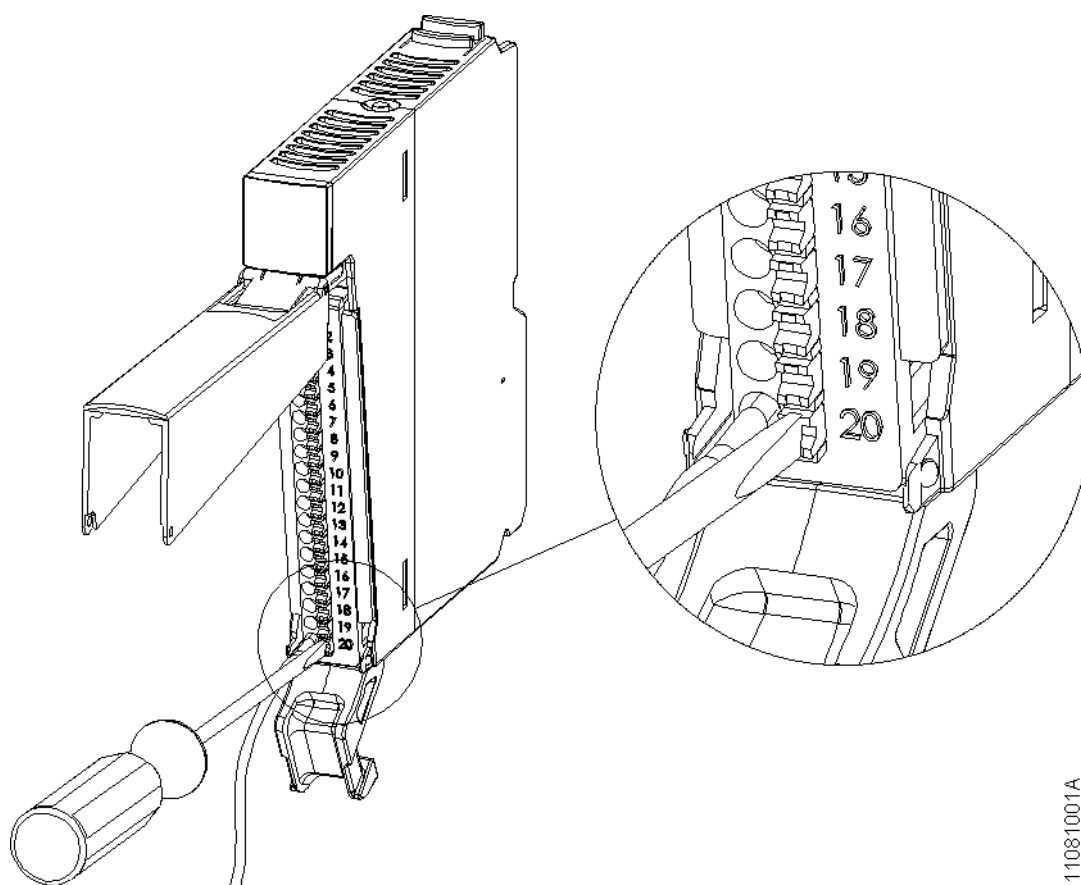
Figure 72: Spring Connection I/O Module
