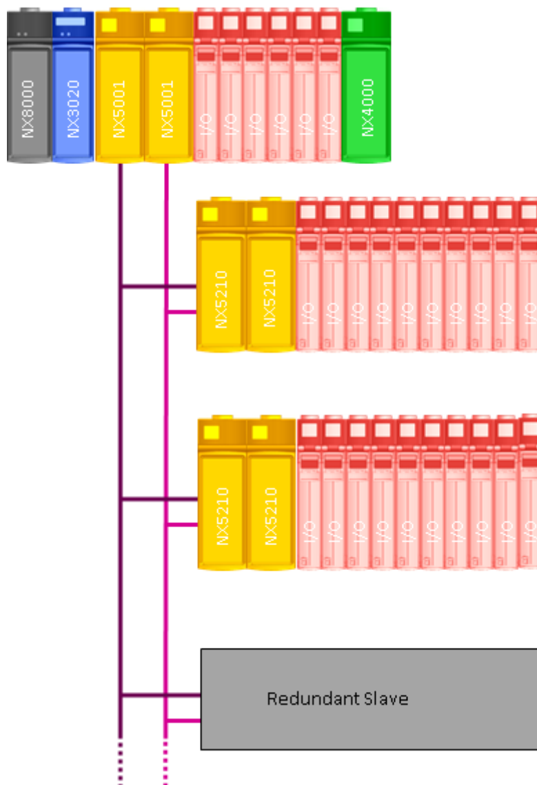
Figure 12: Fieldbus Interfaces with Redundancy
